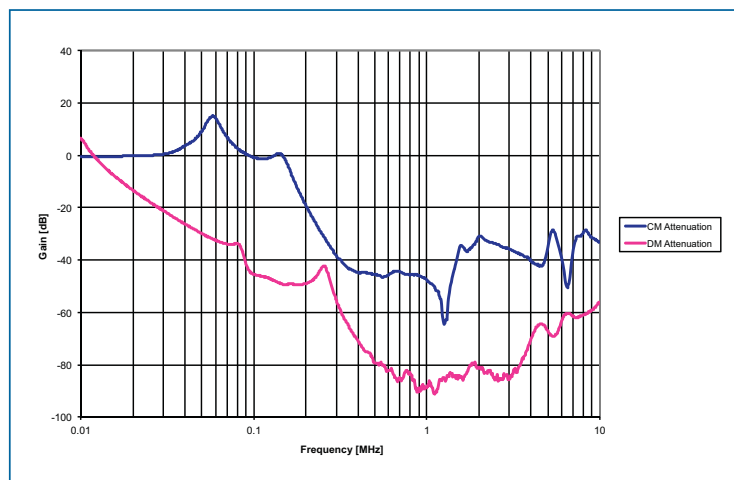
Figure 3 — MF028AMFPT insertion loss
