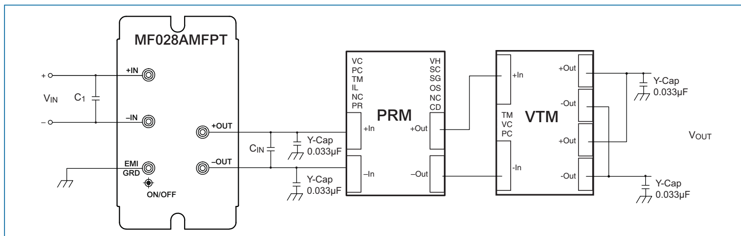
Figure 7 — Recommended circuit for EMI
