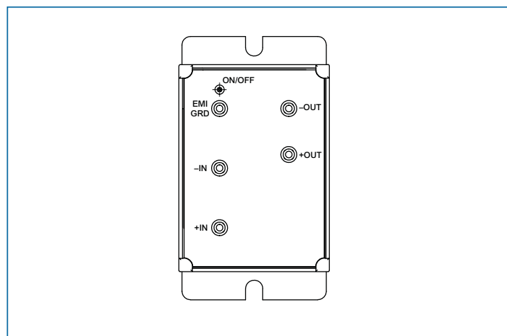
Figure 2 — MF028AMFPT pin configuration (viewed from pin side)
