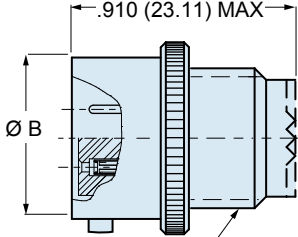
Accessory Thread 803-004-01
