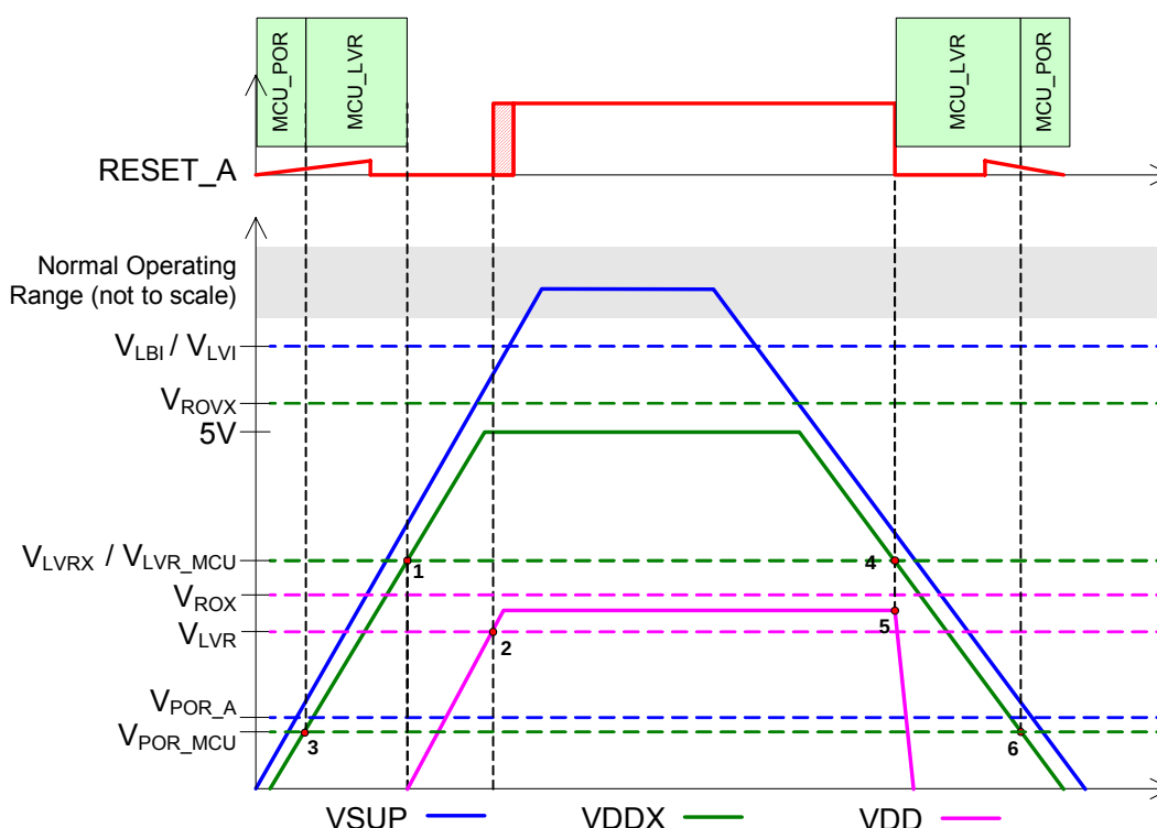
Figure 19. Power Up / Down Sequence
