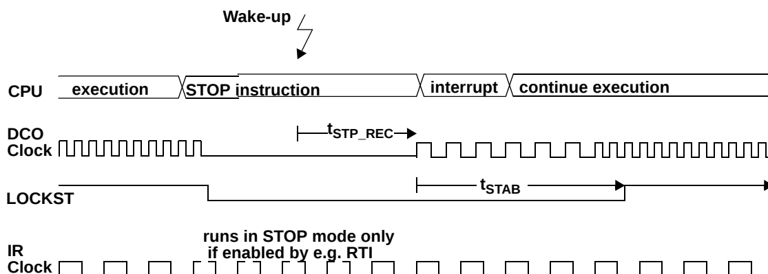
Figure 74. Example of STOP Mode Using DCO Clock as Bus Clock
