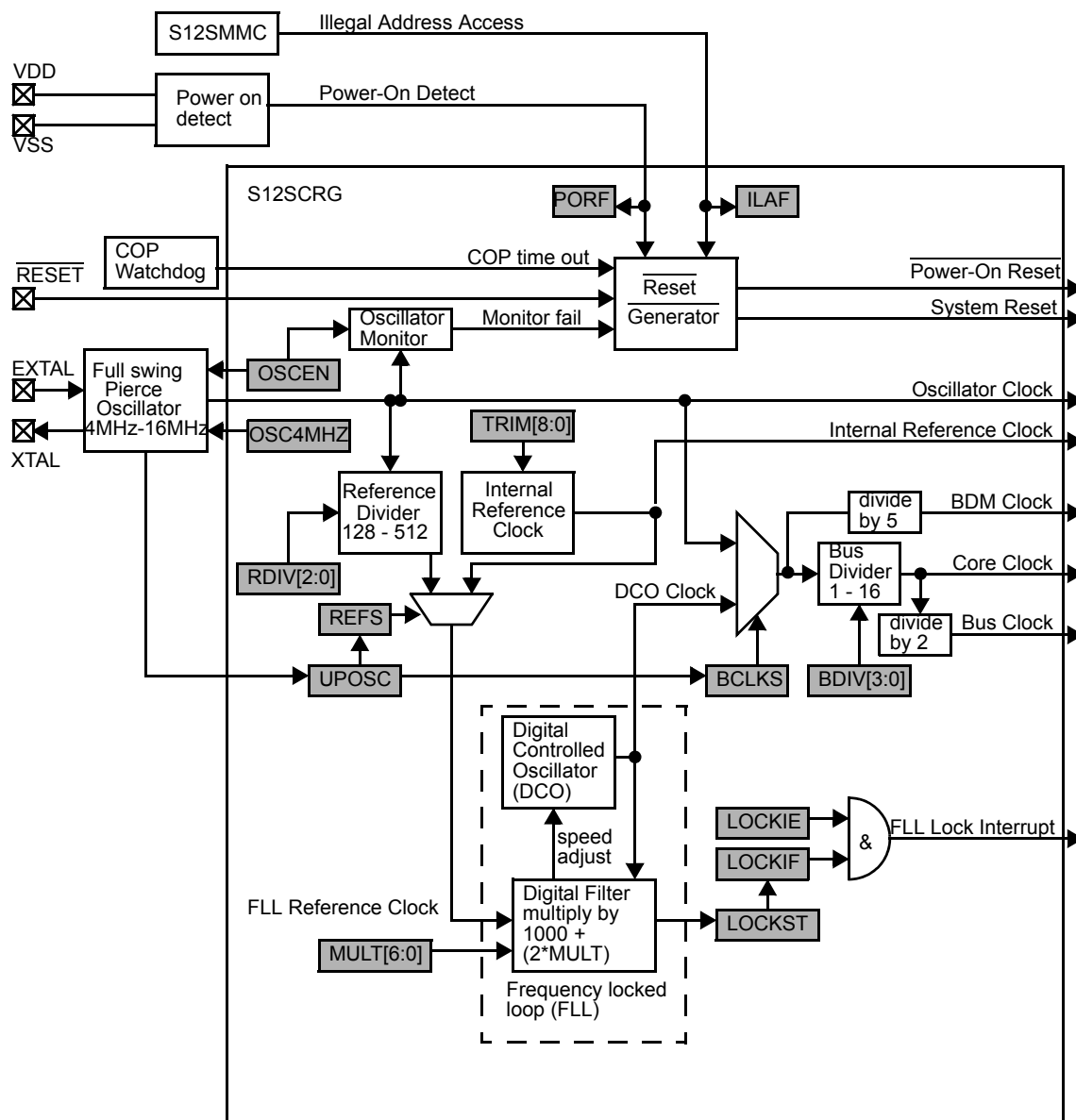
Figure 72. Block diagram of 9S12L32PIMV1
