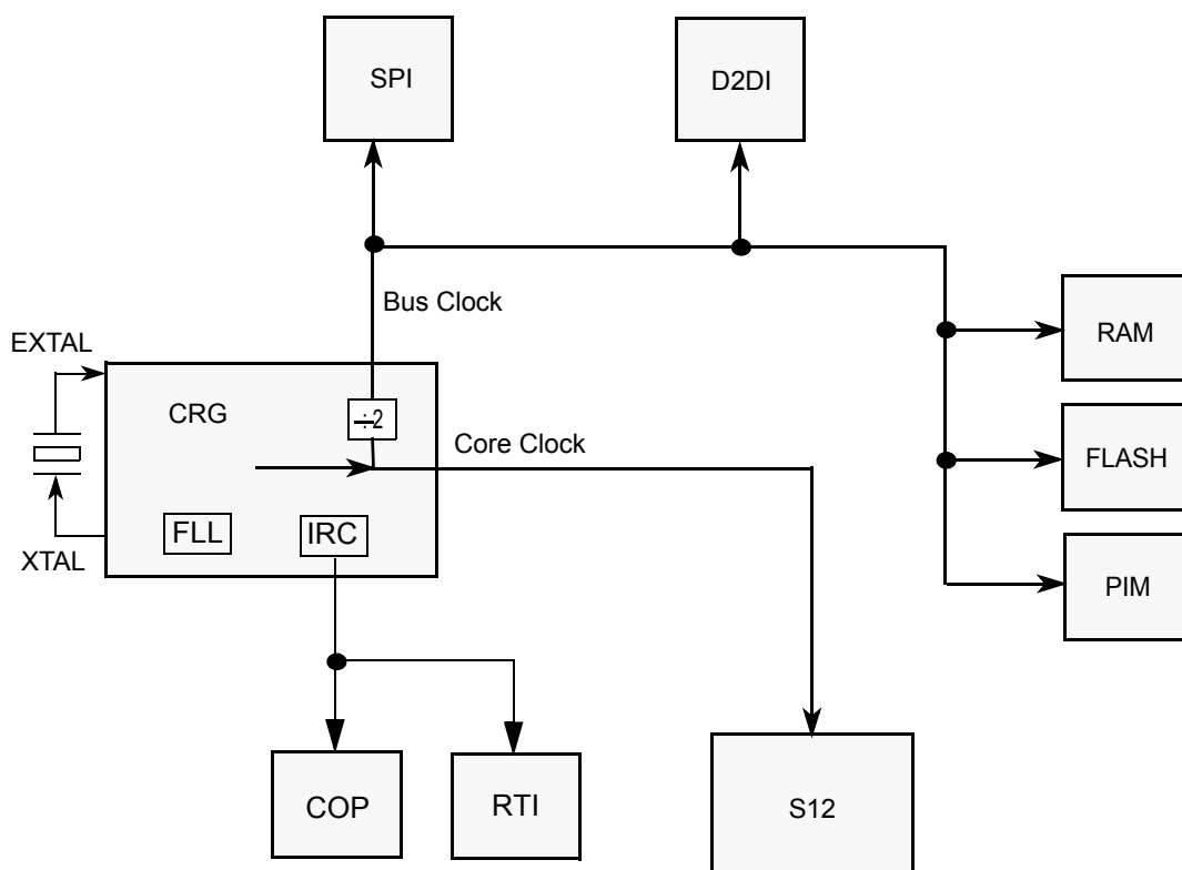
Figure 45. Clock Connections
