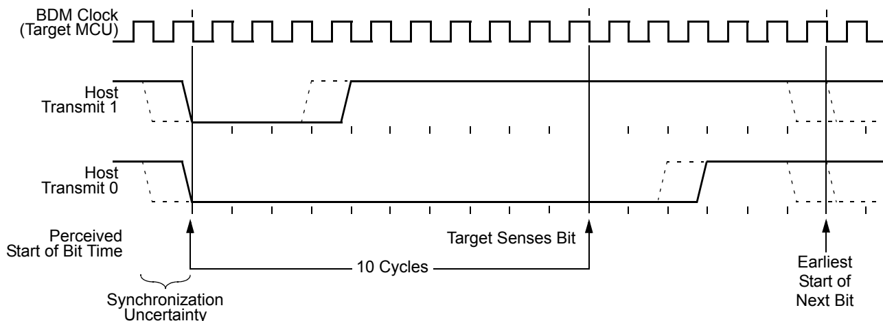
Figure 62. BDM Host-to-Target Serial Bit Timing
