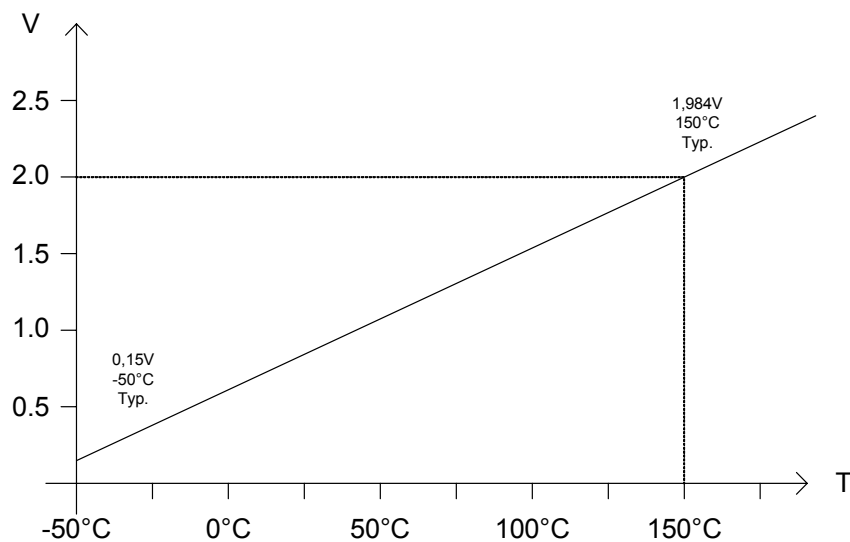
Figure 40. TSENSE - Graph
