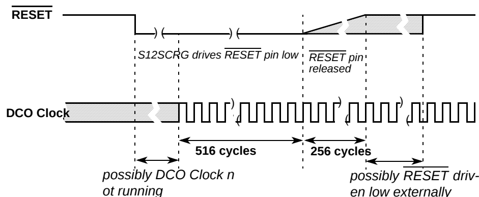
Figure 77. \overline{\text{RESET}} Timing
