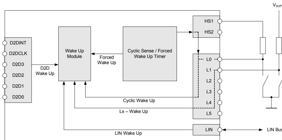
Figure 20. Wake-up Sources
