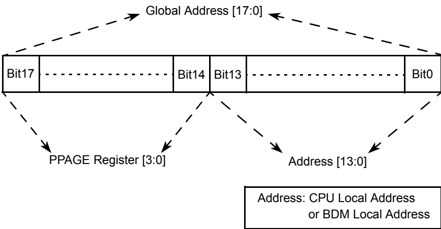
Figure 49. PPAGE Address Mapping
