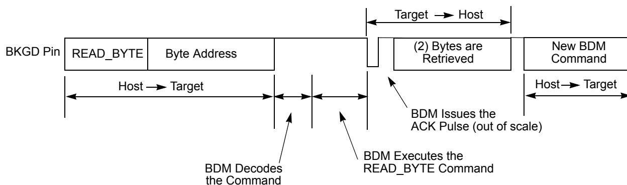
Figure 66. Handshake Protocol at Command Level
