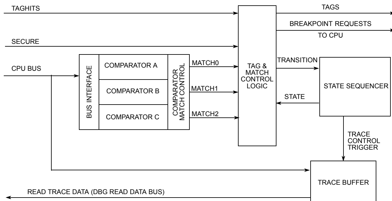
Figure 70. DBG Overview
