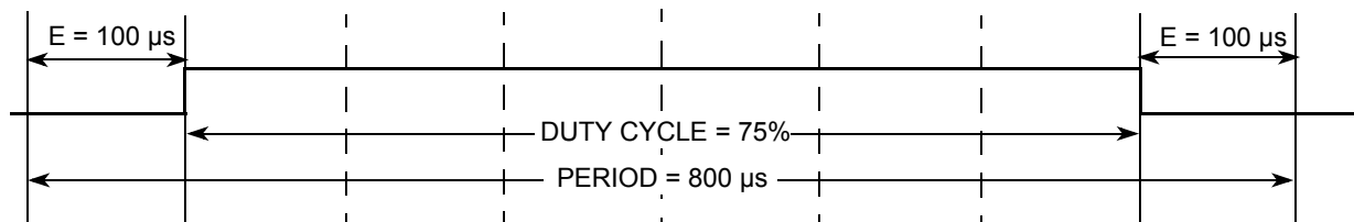
Figure 30. PWM Center Aligned Output Example Waveform
