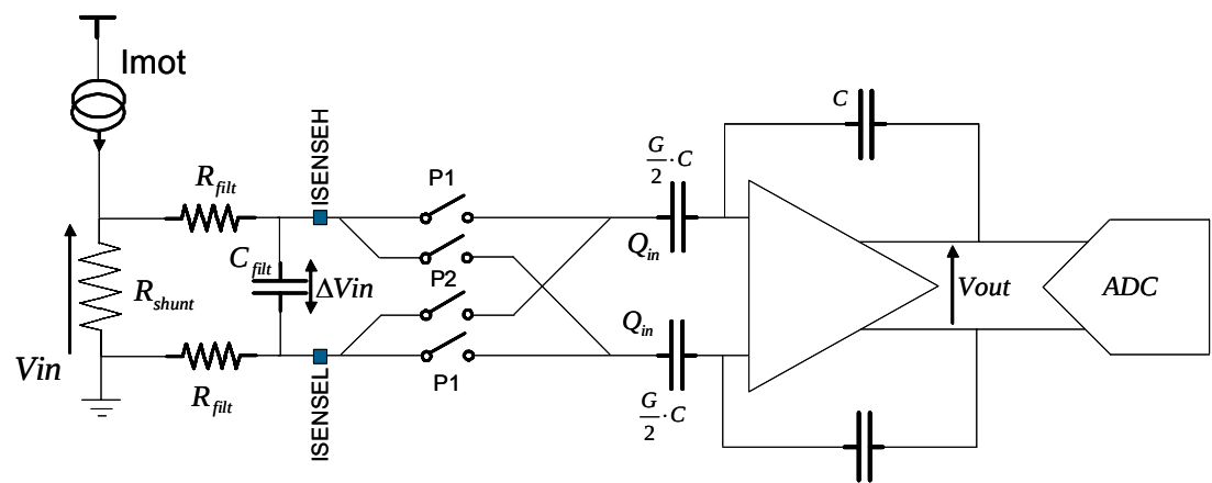
Figure 39. Current Sense Module with External Filter Option
