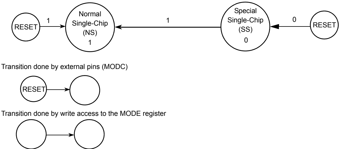
Figure 51. Mode Transition Diagram when MCU is Unsecured
