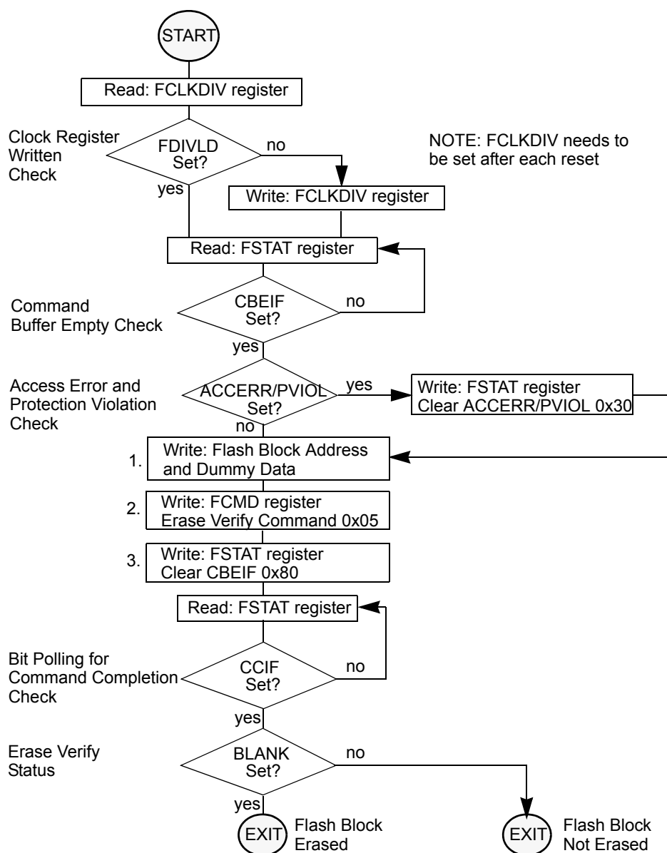
Figure 86. Example Erase Verify Command Flow
