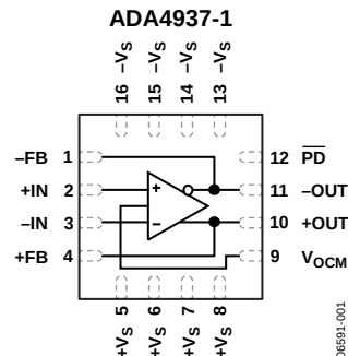
Figure 1. ADA4937-1
