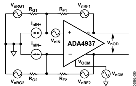
Figure 53. ADA4937-1/ADA4937-2 Noise Model
