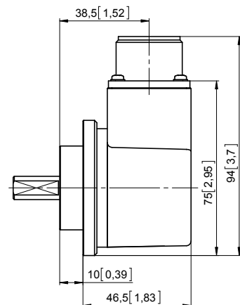
MIL-connector version
