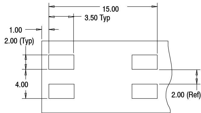
SMT PC Board Layout
