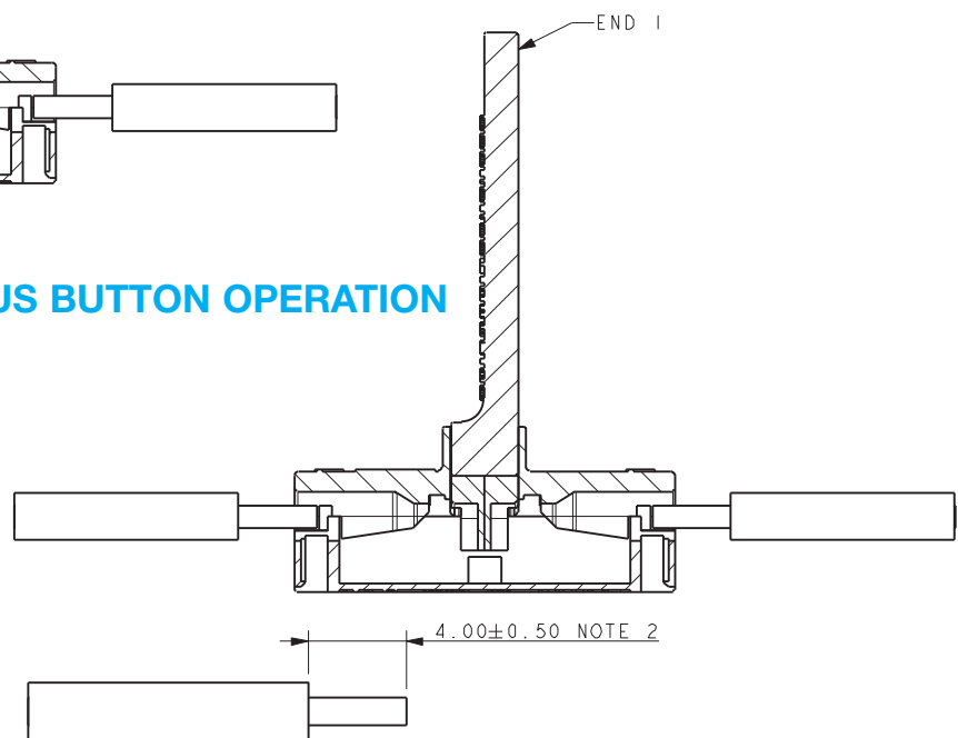
TRIMMED WIRE
