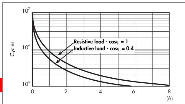
F 48 - Electrical life (AC) v contact current Types 48.52
