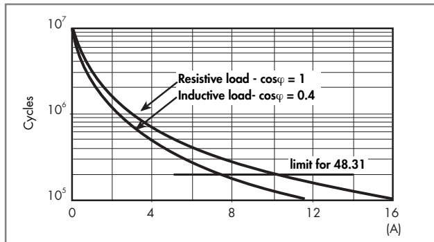
F 48 - Electrical life (AC) v contact current Types 48.31/61
