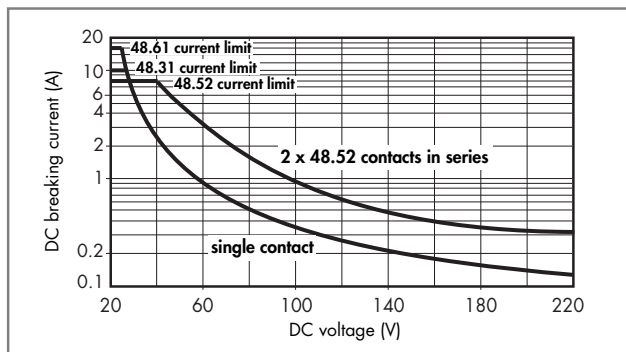
H 48 - Maximum DC1 breaking capacity Types 48.31/52/61
