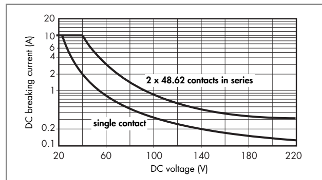
H 48 - Maximum DC1 breaking capacity Type 48.62
