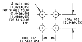
RECOMMENDED HOLE PATTERN GAUGE
