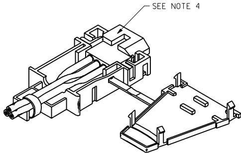
3-CIRCUIT PART (OPEN) (NO SCALE)
