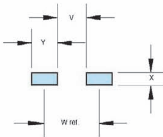
Land Pattern
