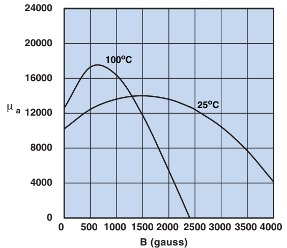
Amplitude Permeability vs. Flux Density
