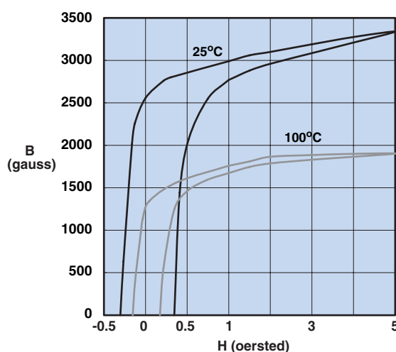
Hysteresis Loop
