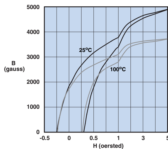
Hysteresis Loop
