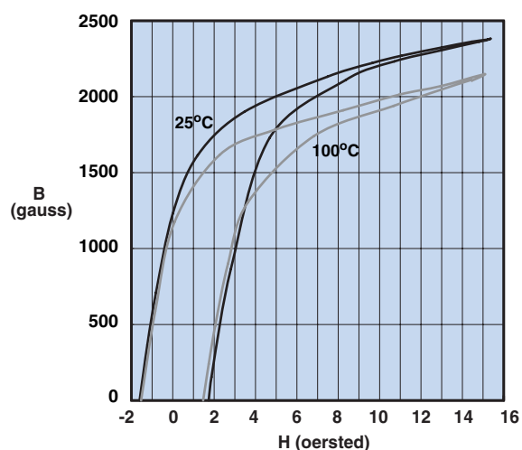
Hysteresis Loop
