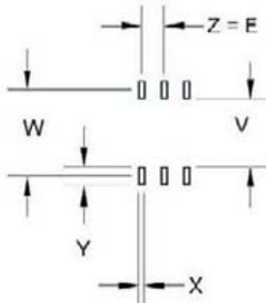
Land Pattern
