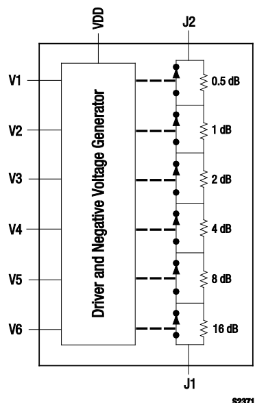
Figure 1. SKY12332-470LF Block Diagram
