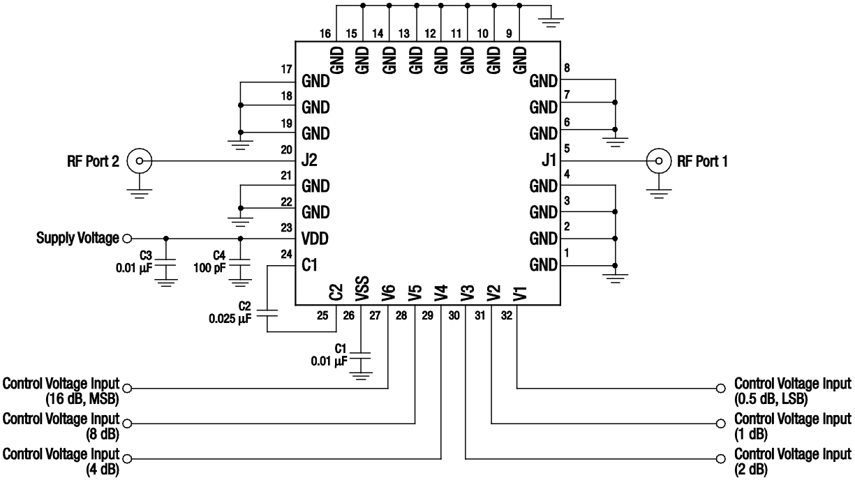
Figure 7. SKY12332-470LF Evaluation Board Schematic Diagram
