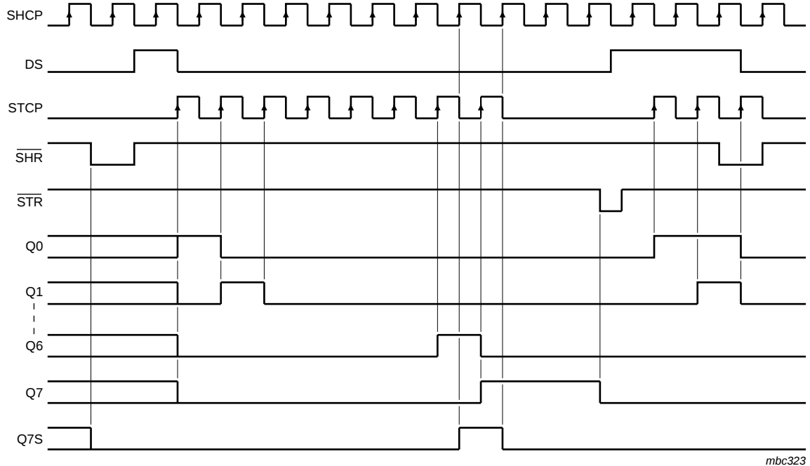
Fig 8. Timing diagram
