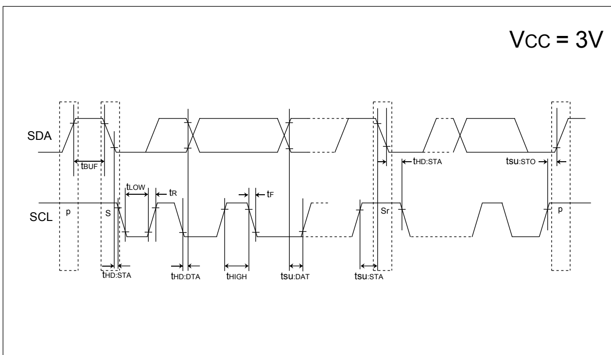
Figure 21.6 Timing Diagram (3)
