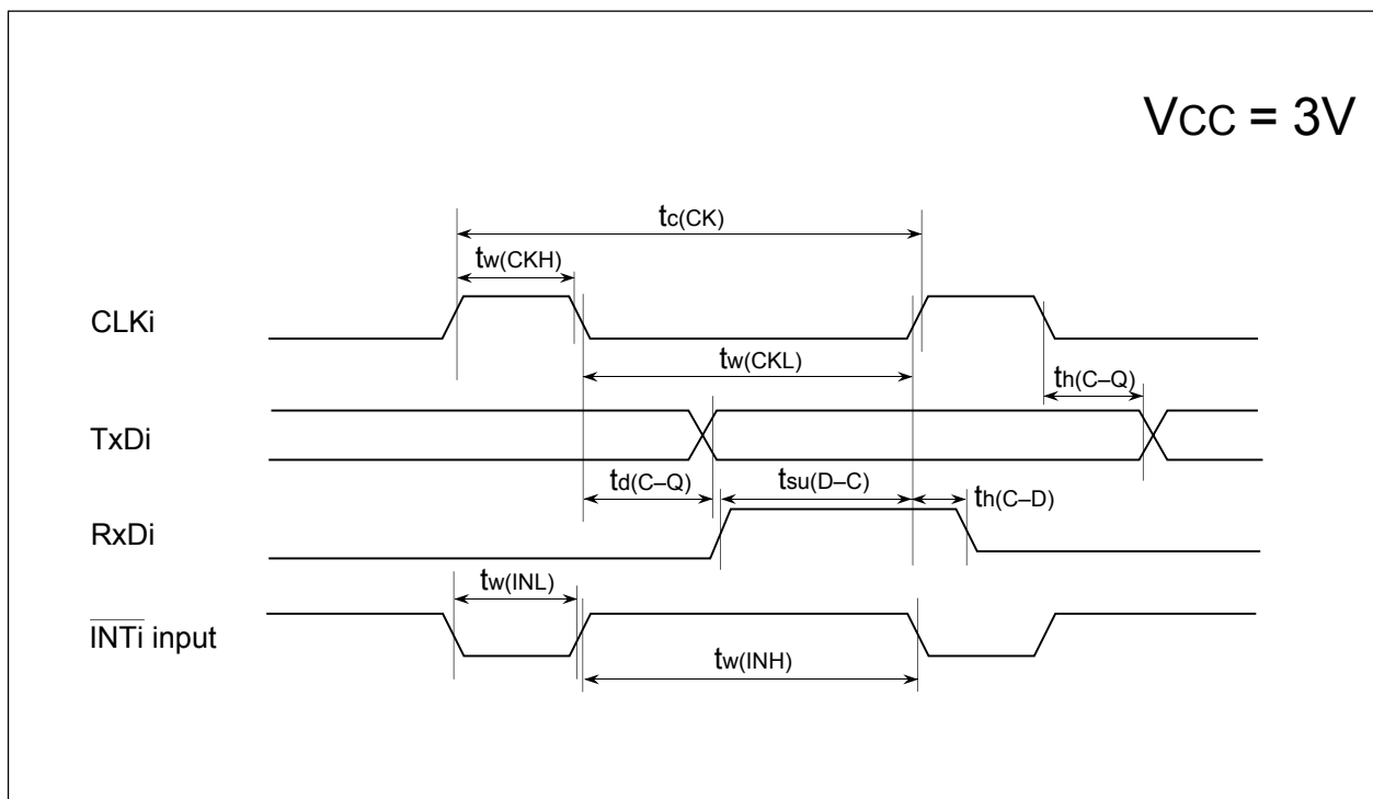
Figure 21.11 Timing Diagram (2)
