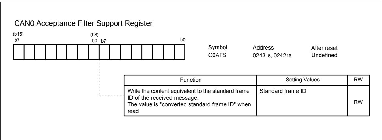
Figure 17.16 C0AFS Register
