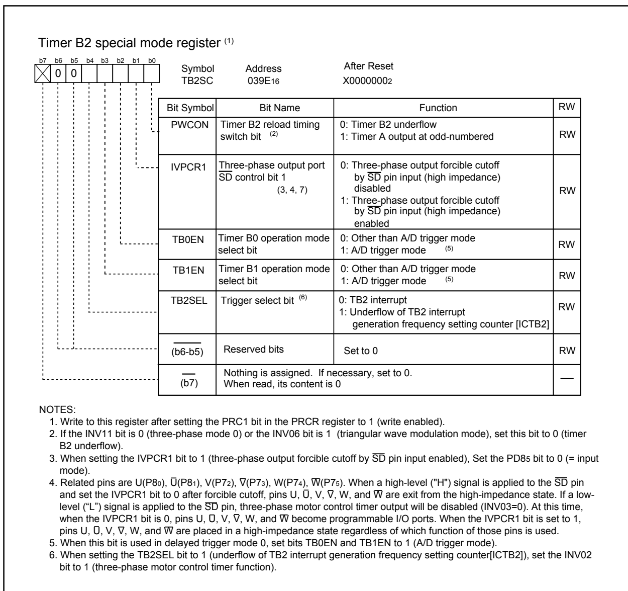
Figure 15.5 TB2SC Register
