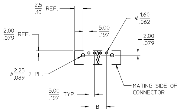
② PCB LAYOUT
