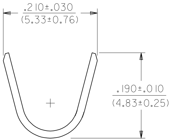
INSULATION CRIMP DETAIL
