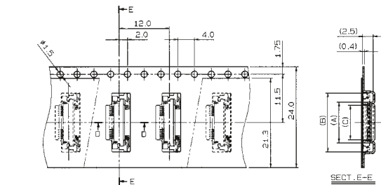
SECT. E-E
