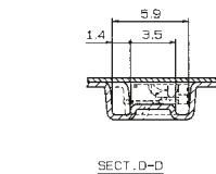
SECT. D-D
