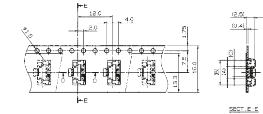
SECT. E-E
