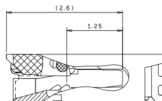
SECT. Y-Y
