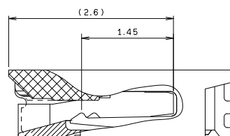
SECT. X-X
