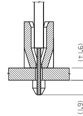
SECT.(CABLE ASS'Y)
