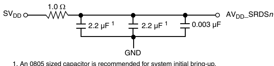
Figure 65. SerDes PLL Power Supply Filter
