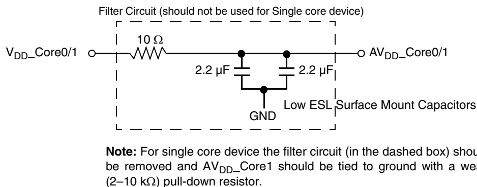
Figure 64. MPC8640 PLL Power Supply Filter Circuit (for cores)
