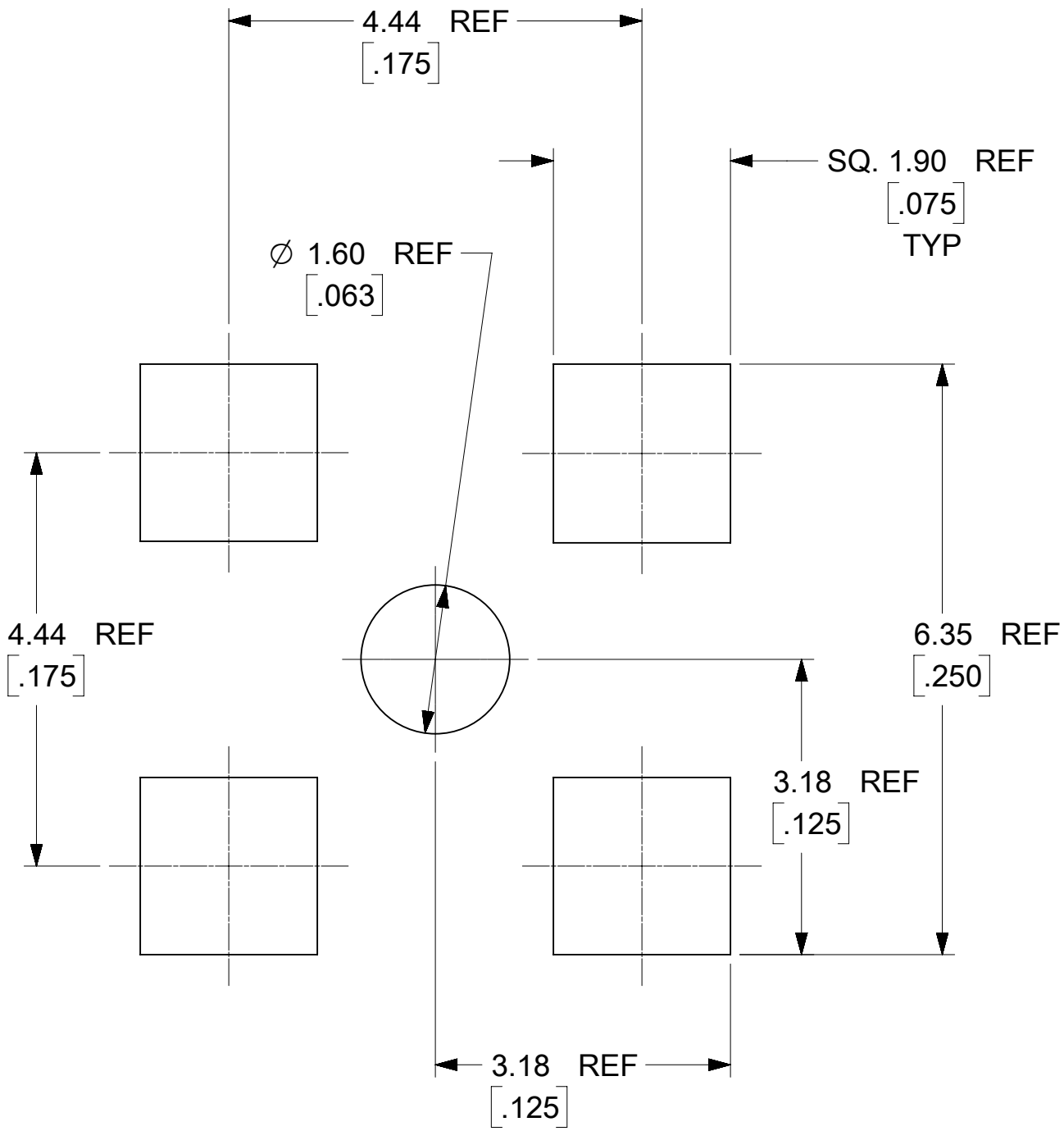
RECOMMENDED MOUTING PATTERN
