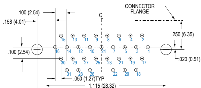
31 SOCKET M83513/13-E
