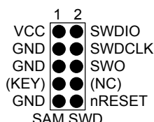
Figure 5-4. Recommended ARM SWD/JTAG Header Pinout
