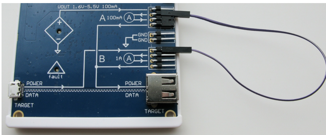
Figure 6-6. Jumper Configuration
