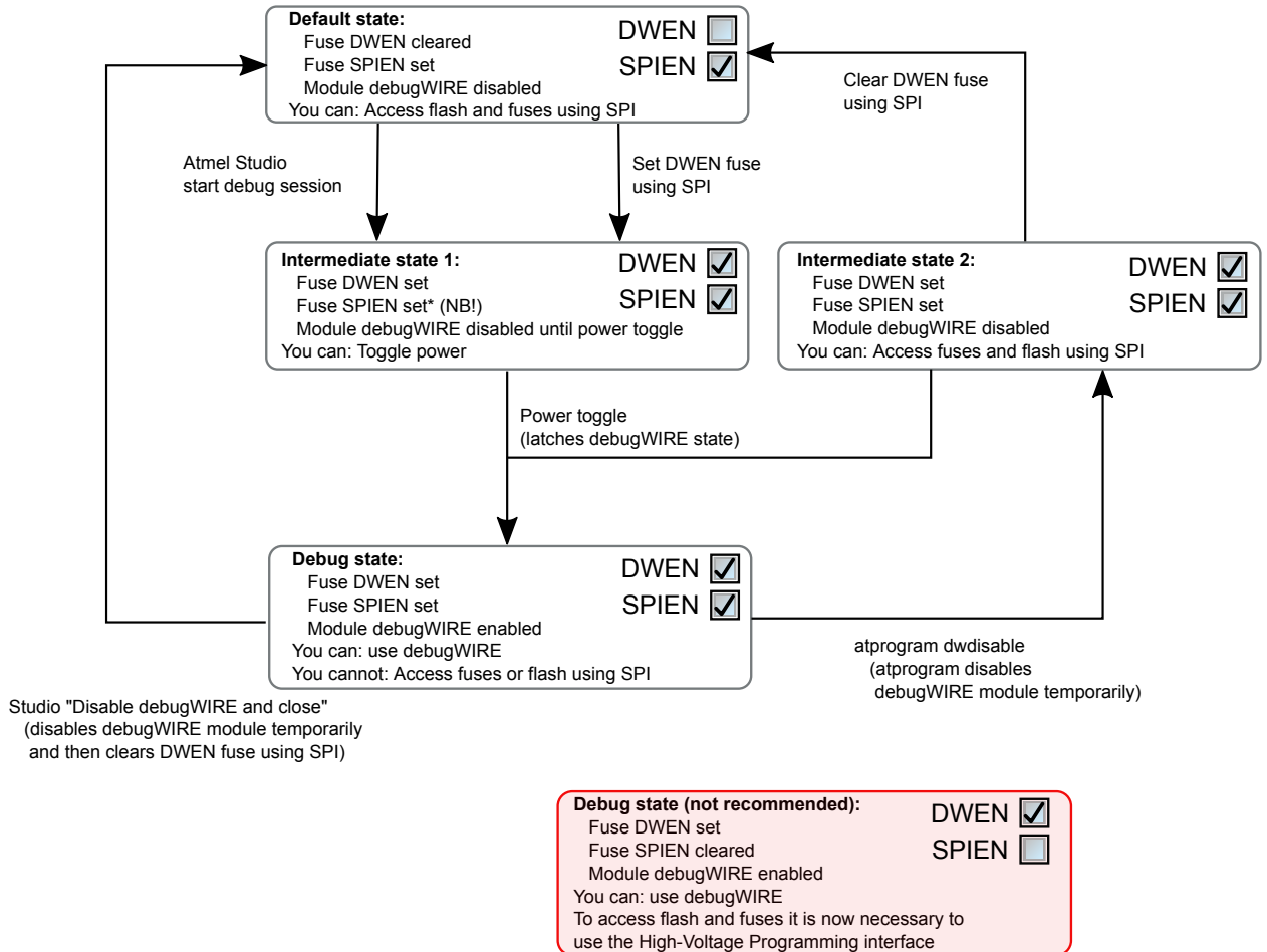
Figure 5-13. Understanding debugWIRE and the DWEN fuse
