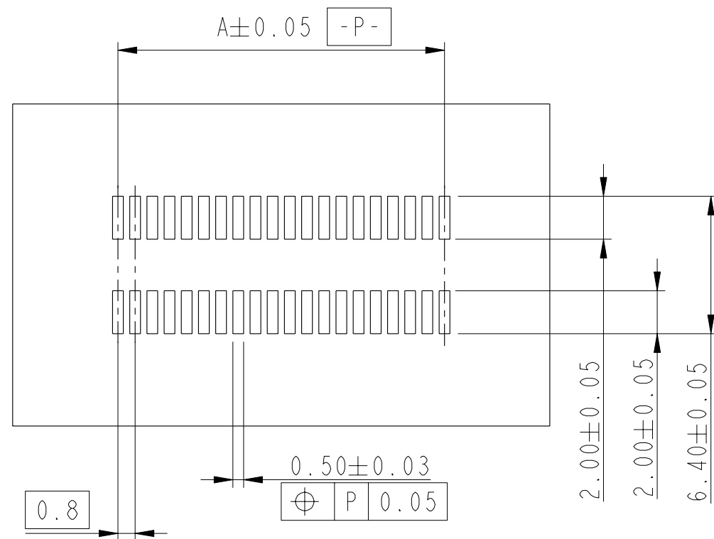
RECOMMENDED PCB LAYOUT WITHOUT PEGS AND HOLDDOWN
