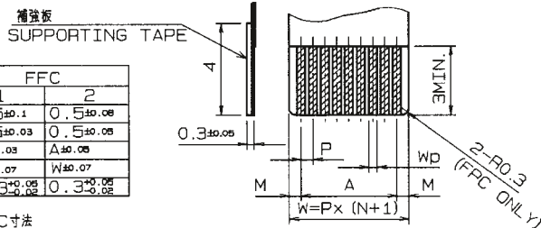
適用FPC, FFC寸法 APPLICABLE FPC, FFC
