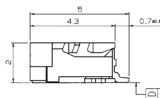
SECT X-X
