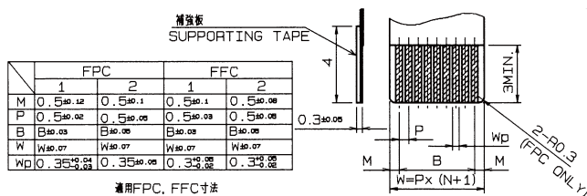
適用FPC, FFC寸法 APPLICABLE FPC, FFC
