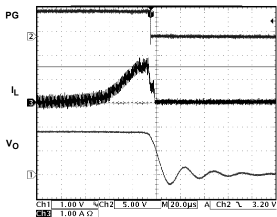
FIGURE 28. OVERCURRENT SHUTDOWN
