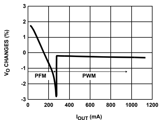
FIGURE 24. PFM-PWM TRANSITION
