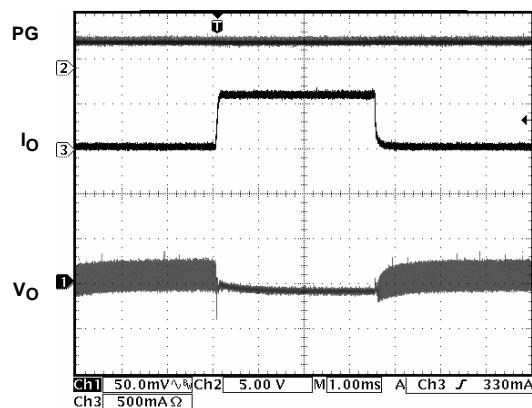
FIGURE 25. PFM-PWM LOAD TRANSIENT
