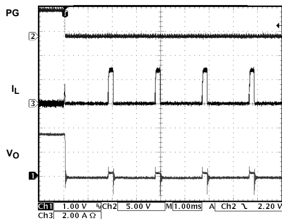
FIGURE 29. OVERCURRENT HICCUP MODE
