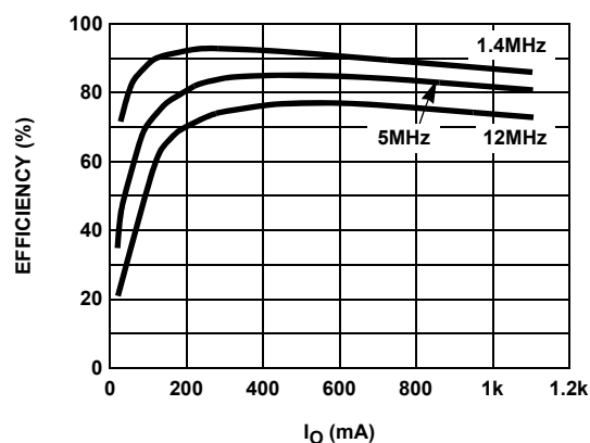
FIGURE 19. EFFICIENCY vs I_O (PWM MODE)
