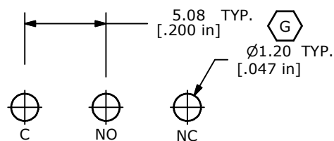
P.C. MOUNTING
