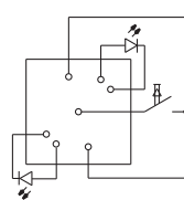
Keyswitch, spot-illuminated
