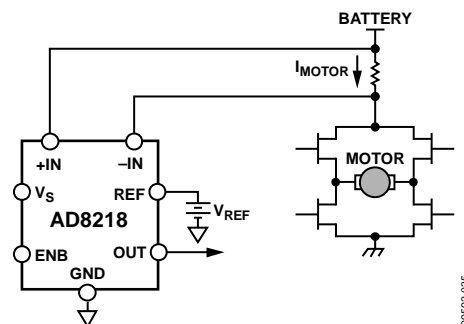
Figure 36. High-Side Current Sensing in Motor Control
