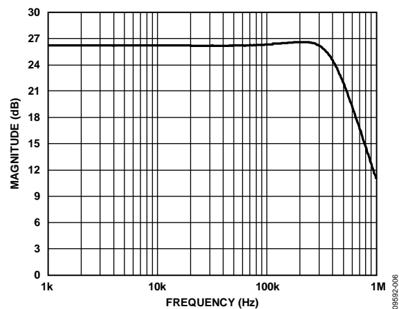
Figure 7. Typical Small-Signal Bandwidth ( V_{OUT} = 200\text{ mV p-p} )
