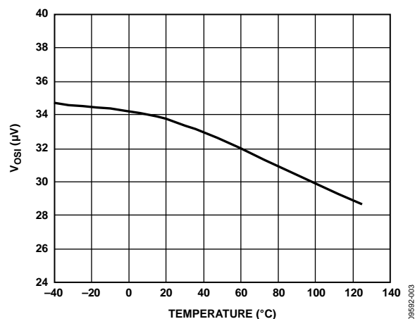
Figure 4. Typical Input Offset vs. Temperature
