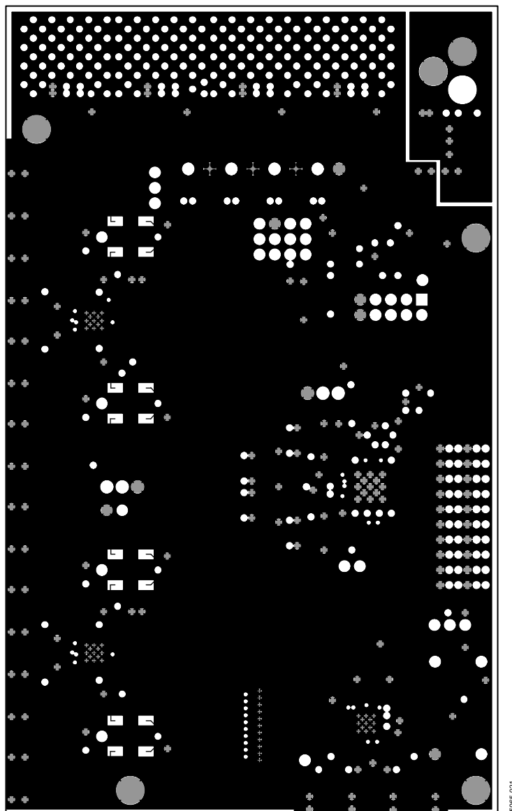
Figure 68. Evaluation Board Layout, Ground Plane
