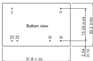
Standard pinning
