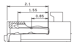
SECT. X-X
