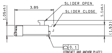
SECT. X-X
