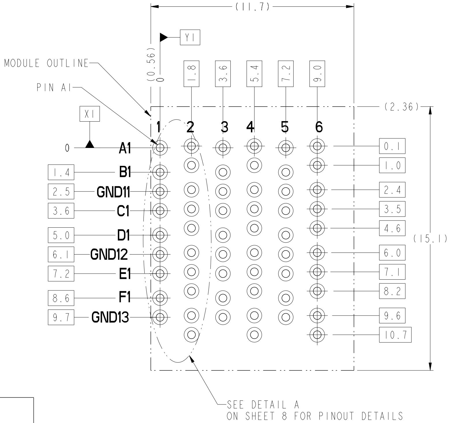
RIGHT WALL MODULE BACKPLANE FOOTPRINT
