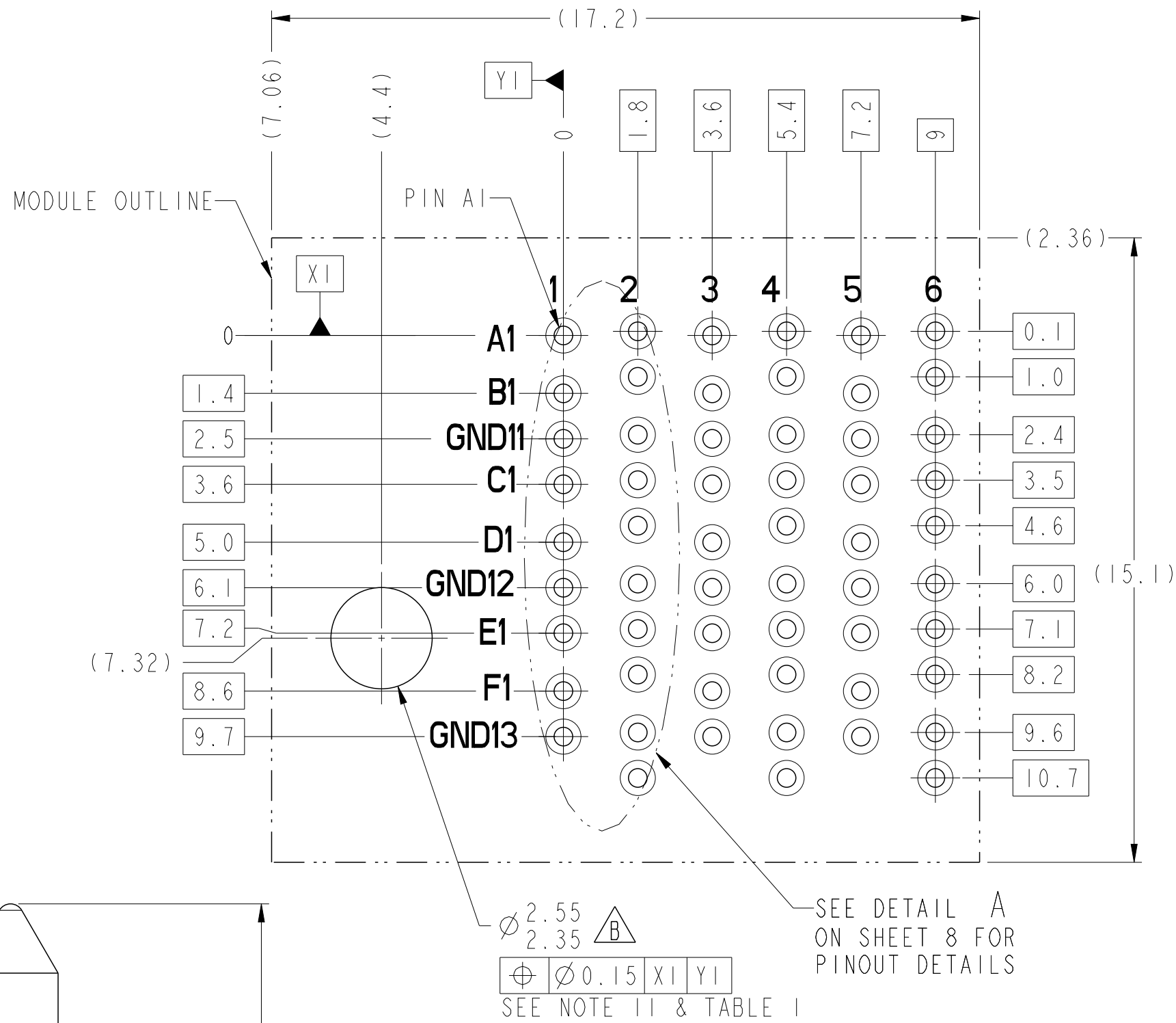
BP HOLE PATTERN COMPONENT SIDE LEFT POLARIZING / GUIDE MODULE BACKPLANE FOOTPRINT
