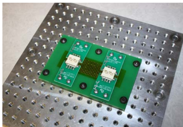
Figure 3- Vibration fixture
