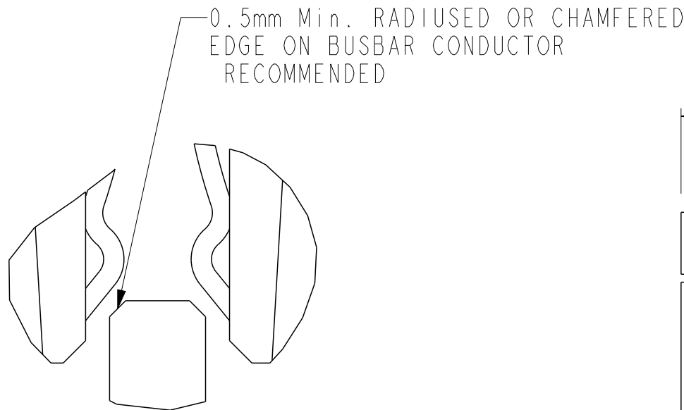
DETAIL A (6:1)
