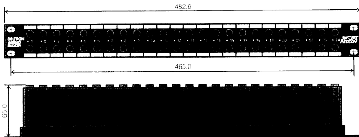
TYPICAL PATCHBAY ASSEMBLY
