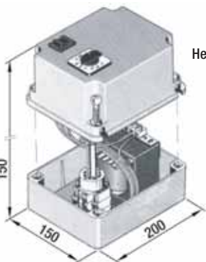
Single-phase speed setting for wall assembly (with 5 steps)
