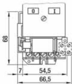
Motor protection switch for assembly inside a cabinet (3-phase current)
