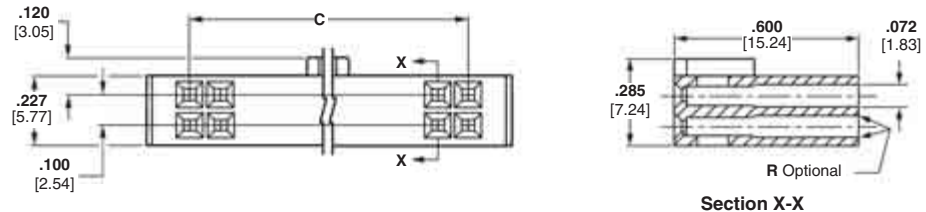
Section X-X
