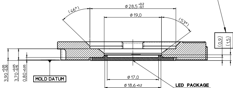
SECTION W-W
