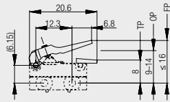
L41: adjustable plastic lever 190.075.013
