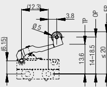
L43: adjustable roller lever 190.072.013
