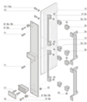
Item 8b, 6 U front panel mounting
