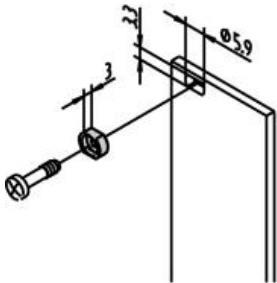
Front panel fixing
