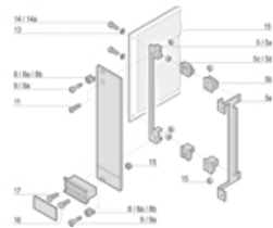
Item 8b, 3 U front panel mounting
