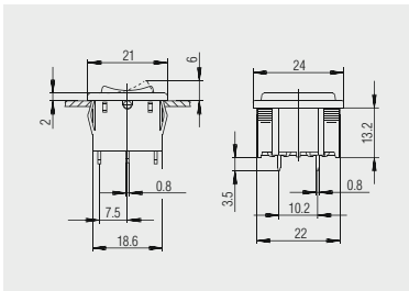
PCB terminal
