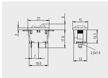
Solder terminal basic type 1808
