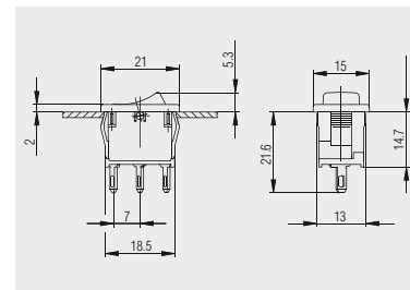
Solder terminal basic type 1800
