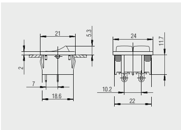
Solder terminal 1806.6108
