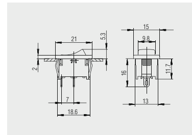
Solder terminal basic types 1801 and 1803
