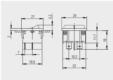
Quick-connect terminal 4.8 x 0.8 1806.2054 and 1806.1102
