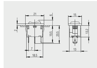
Quick-connect terminal 4.8 x 0.8 basic type 1808
