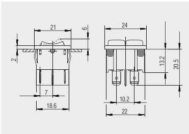
Quick-connect terminal 4.8 x 0.8 1806.1602
