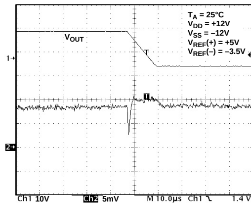
Figure 17. DAC-to-DAC Crosstalk
