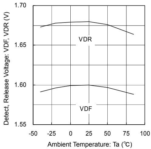
XC61X1~XC61X7 (1.6V)
