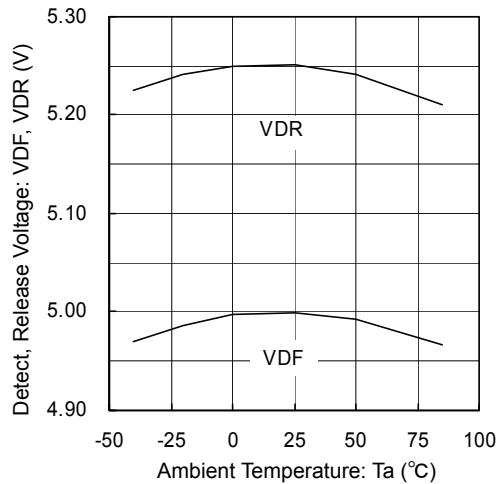
XC61X1~XC61X7 (5.0V)
