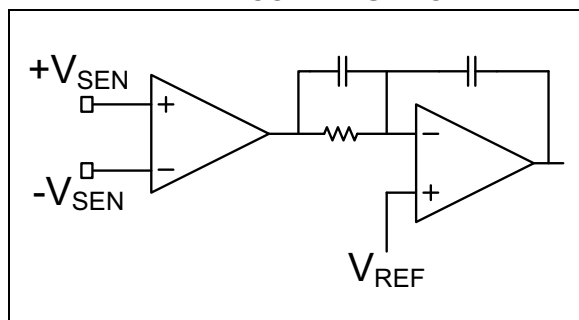
FIGURE 3-1: SIMPLIFIED INTERNAL COMPENSATION
