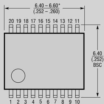
F Package 20-Lead Plastic TSSOP (4.4mm) (LTC DWG # 05-08-1650)
