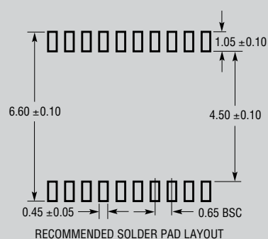
F Package 20-Lead Plastic TSSOP (4.4mm) (LTC DWG # 05-08-1650)
