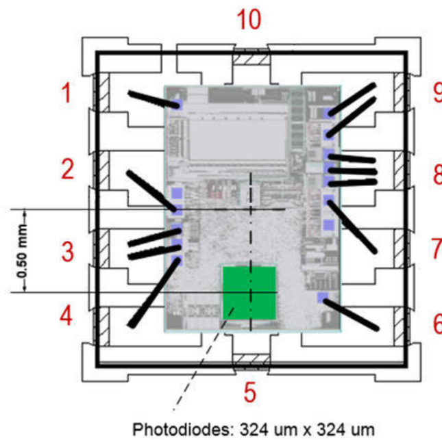
Figure 7.2. Photodiode Locations
