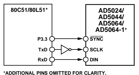
Figure 54. AD5024/AD5044/AD5064/AD5064-1 to 80C51/80L51 Interface
